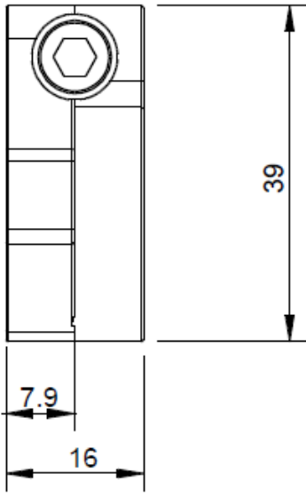
Flanged Shaft Support 20mm
