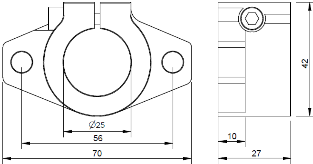
Flanged Shaft Support 25mm
