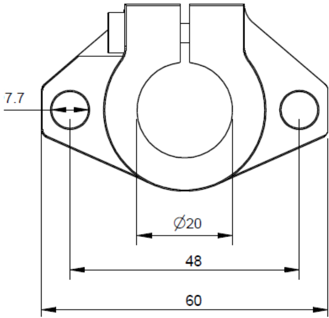
Flanged Shaft Support 20mm
