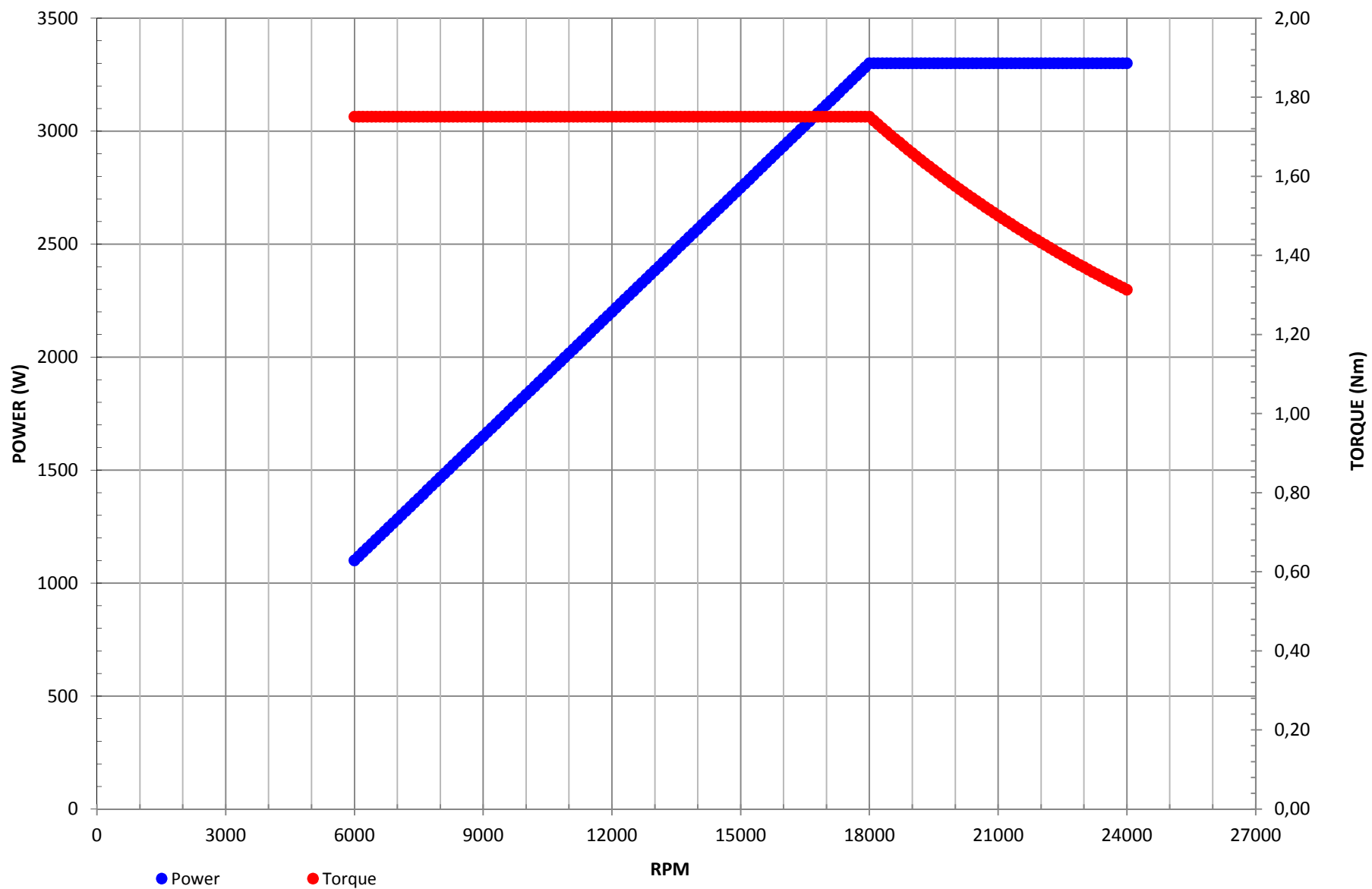
Torque & Power Curve C51/60-A-DB-P-ER32-HY-3.3KW-18000-24000RPM
